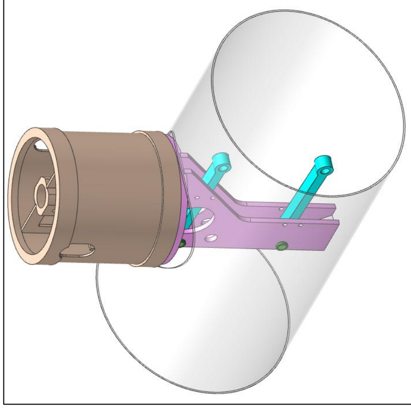
Fig. 20 Guide support part
