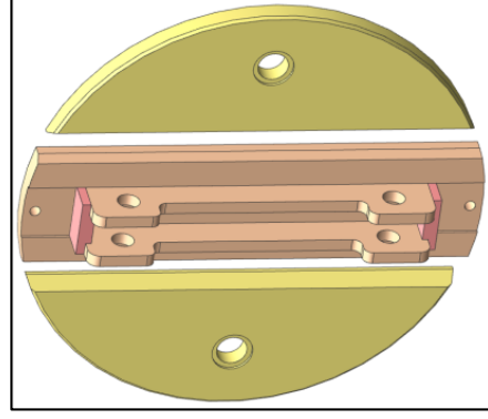
Fig. 3 Element plate
