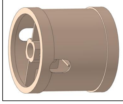
Fig. 21 Guide support
